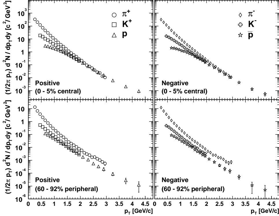
Fig. 11. Transverse momentum distributions for pions, kaons, protons, and anti-pions in Au+Au collisions at \sqrt{s_{NN}} = 200 GeV [54].
